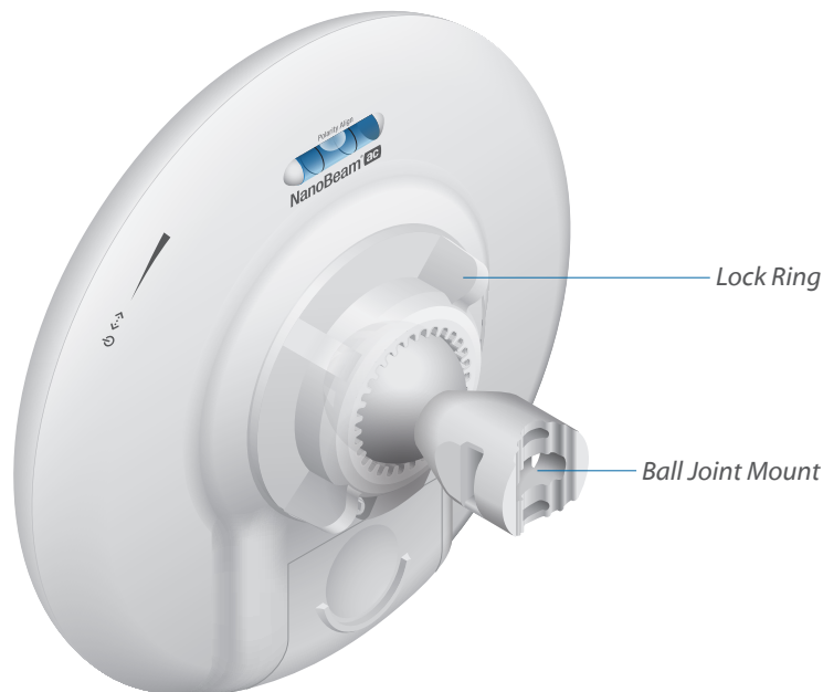
NBE-5AC-19 with Mounting Hardware
